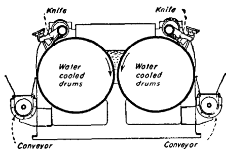
FIG 7 - DOUBLE-DRUM FLAKER
